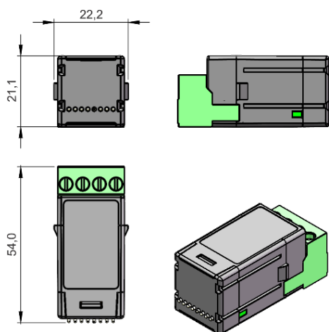
Figure 1 – Module overview
