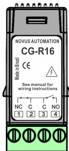
Figure 2 – Electrical connection
